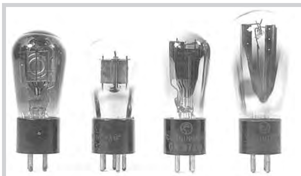
The tubes that made the first true AC sets possible included, from left: UX-226, UY-227, UX-171-A and UX-280.
