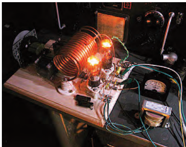
This homebuilt Hartley netted Jim many pleasurable contacts during the Bruce Kelley QSO party.
