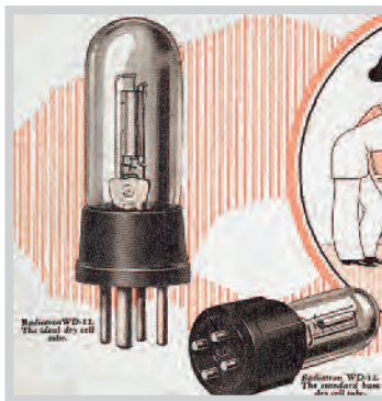
Drawing from RCA ad shows WD-II (upright) and WD-12 tubes. Note fat pin (plate connection) at front of WD-II base.
