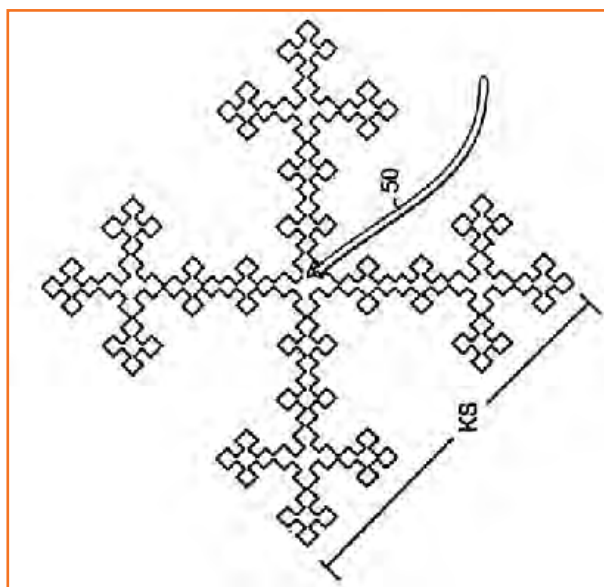
Fractal antenna patent drawing.
