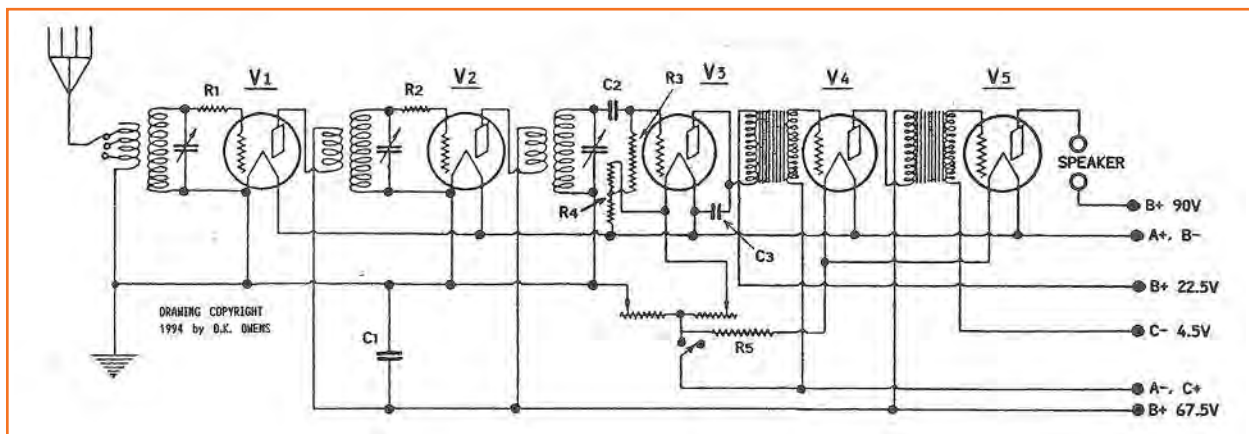
Fig. 1. Schematic of the Atwater Kent Model 20C.
