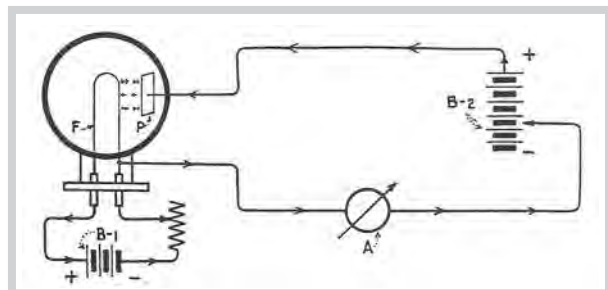
A Fleming Valve demonstration circuit. When an AC source is connected in place of battery B-2, rectification will take place—converting AC to pulsating DC.
