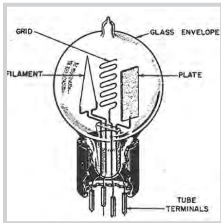
Simplified drawing of de Forest's 3-element "Audion." The original tube had no base.
