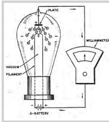
The “Edison Effect” test circuit. Milliammeter indicates current flow through bulb when connected to positive filament lead.
